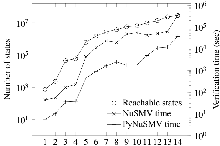
Figure 4: Evolution of number of reachable states and verification time for NuSMV and PyNuSMV in terms of number of considered routes.
