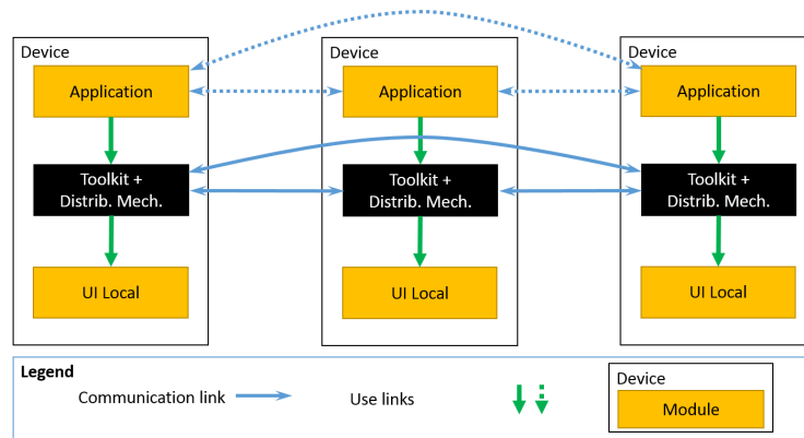
Figure 3.2: The structure of a distributed application
