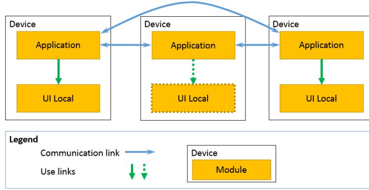
Figure 3.1: The structure of common distributed applications
