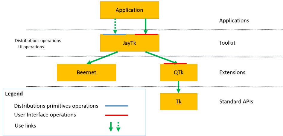
Figure 3.5: The structure of an application using the JayTk
