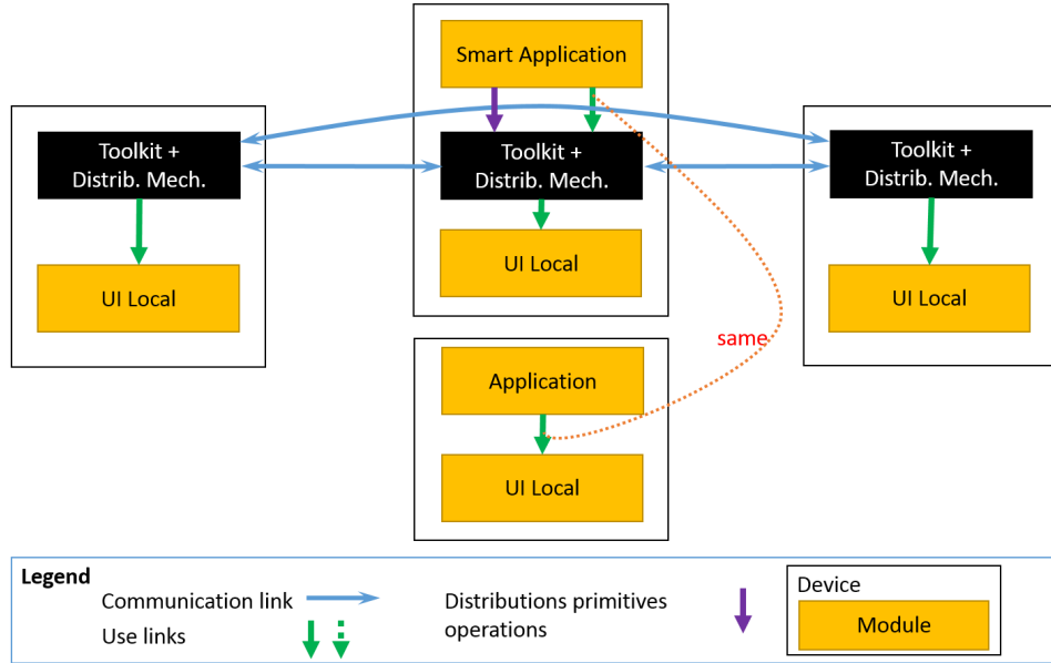
Figure 3.4: An example of a distribution-aware application
