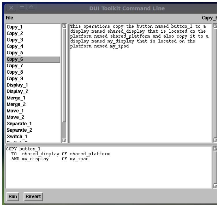
Figure 5.3: Example of a command-line user interface.
