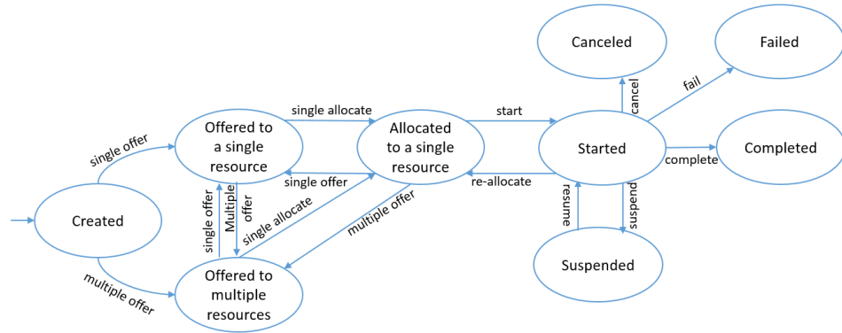
Figure 2.20: A workflow representing the life cycle of a task[RUS05].
