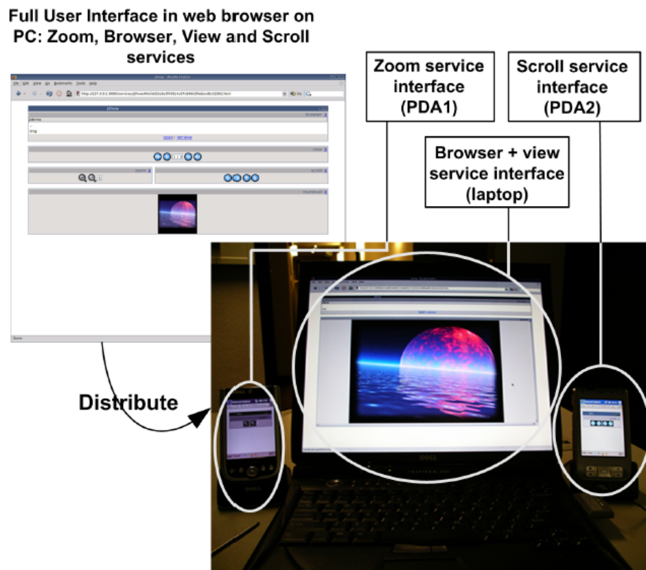
Figure 2.13: An example of website distributed across 3 devices thanks to the Light-weight services[VDV05].
