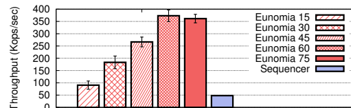
Figure 2: Maximum throughput achieved by Eunomia and an implementation of a sequencer. We vary the number of partitions that propagate operations to Eunomia.
